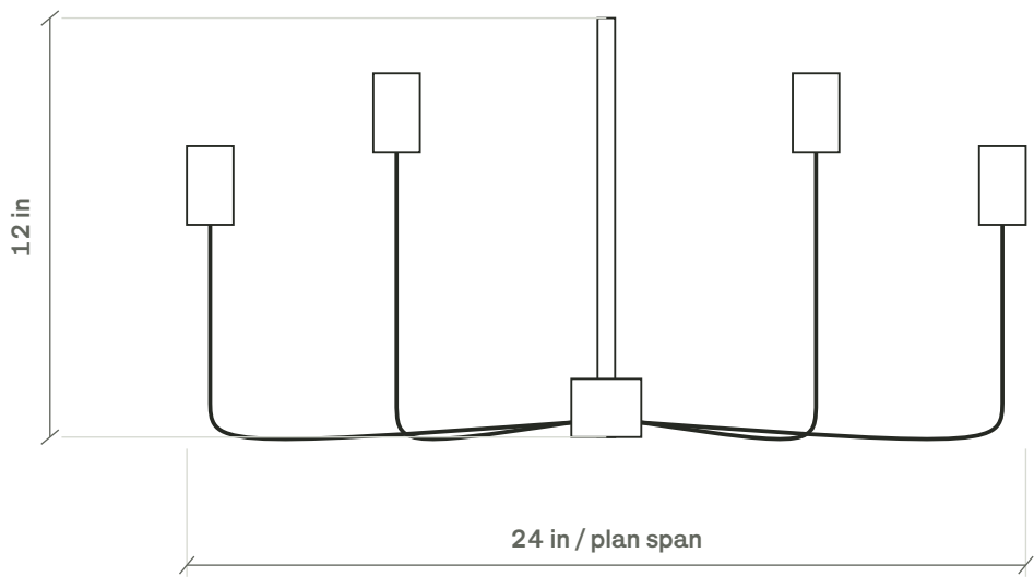
Four-arm layout / bend profiles schematic
