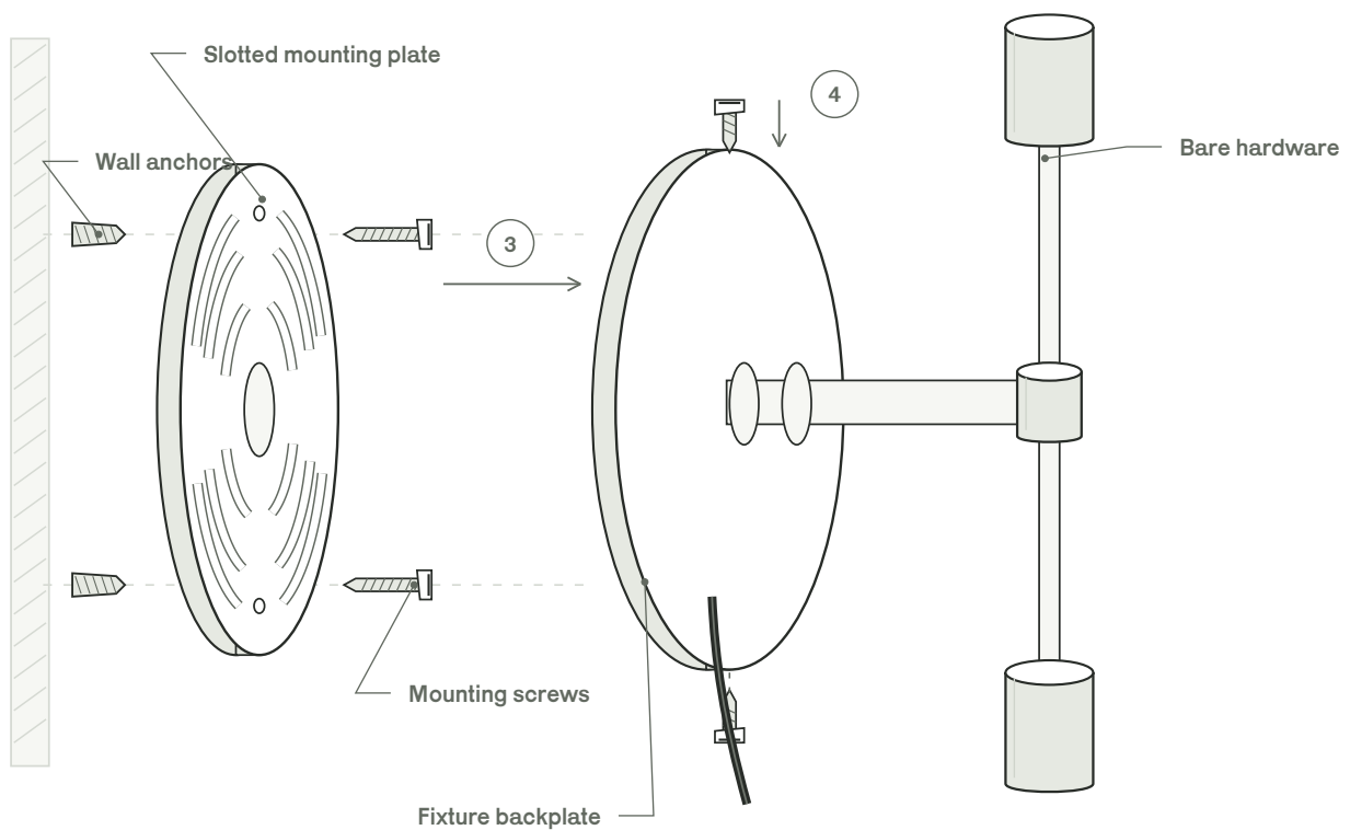
EXPLODED ASSEMBLY / schematic hardware profiles and slot pattern
